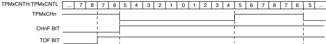
Figure 16-6. Low-True Pulse of a Center-Aligned PWM
