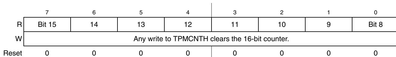
Figure 16-4. Timer Counter Register High (TPMCNTH)
