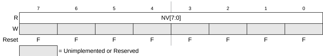
Figure 9-22. Flash Option Register (FOPT)
