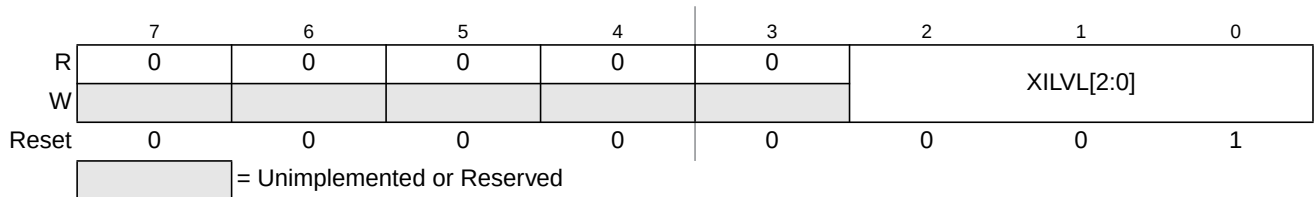
Figure 4-4. XGATE Interrupt Priority Configuration Register (INT_XGPRIOR)
