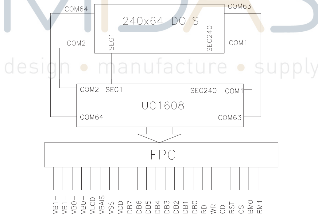
Figure 1. Block diagram
