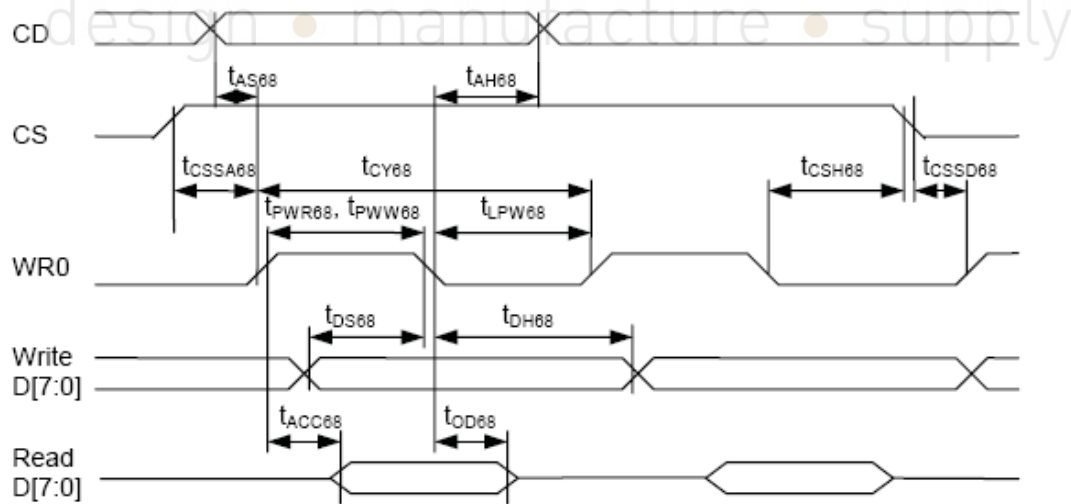
Parallel Bus Timing Characteristics (for 6800 MCU)
