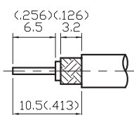
Stripping Dimensions
