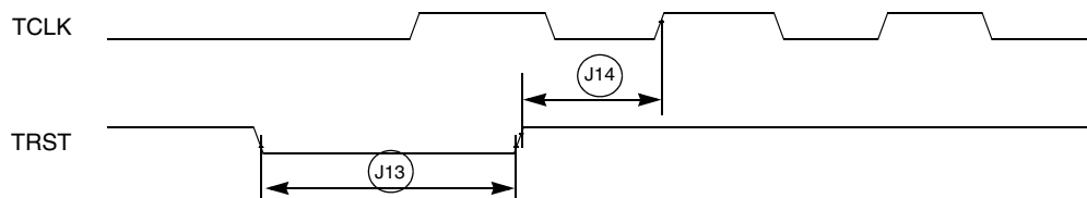
Figure 23. TRST Timing
