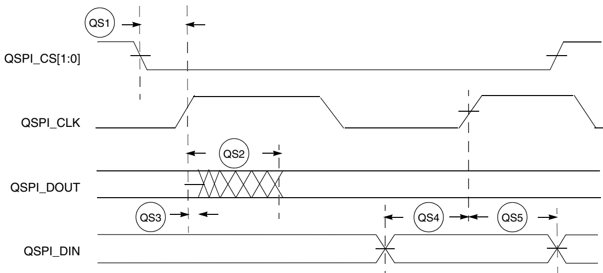
Figure 19. QSPI Timing
