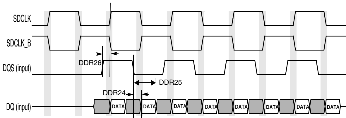
Figure 33. DDR2 SDRAM DQ vs. DQS and \overline{SDCLK} READ Cycle Timing Diagram
