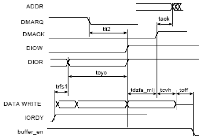
Figure 83. UDMA Out Device Terminates Transfer Timing Diagram
