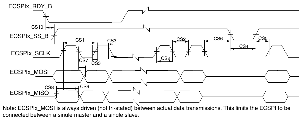
Figure 41. ECSPi Master Mode Timing Diagram
