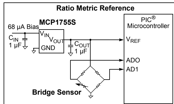
FIGURE 5-2: Using the MCP1755/1755S as a Voltage Reference.
