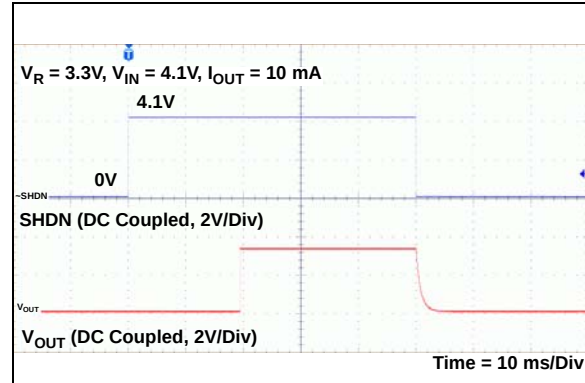
FIGURE 2-34: Start-up from \overline{\text{SHDN}} ( V_R = 3.3\text{V} ).
