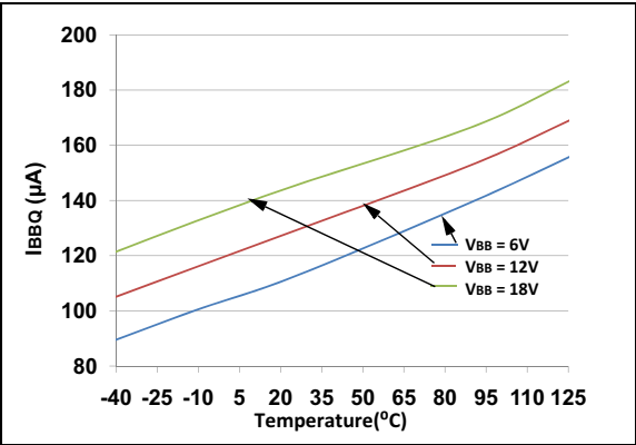
FIGURE 2-8: TYPICAL I BQ VS. TEMPERATURE - 3.3V
