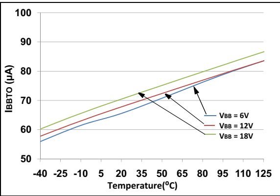
FIGURE 2-9: TYPICAL I BBT0 VS. TEMPERATURE - 3.3V
