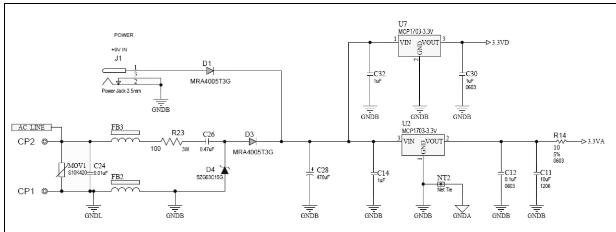
FIGURE 8-3: Power Supply with Separate Lines for Analog and Digital Sections. Note the "Net Tie" Object NT2 that Represents the Star Ground Connection.
