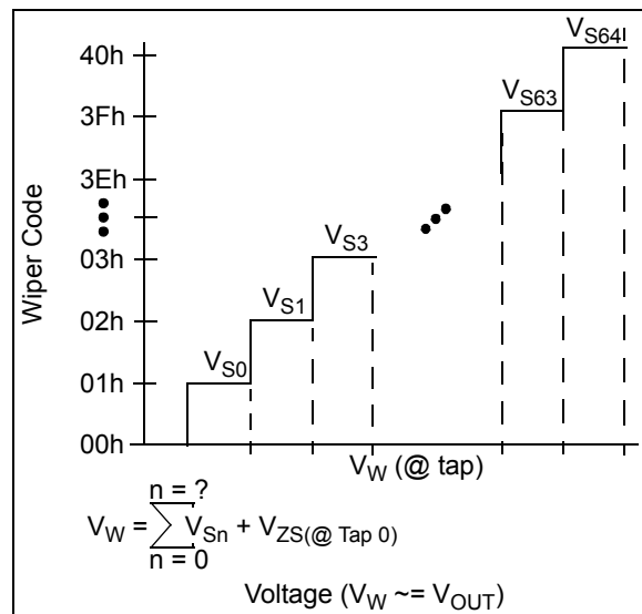
FIGURE C-1: V_W (V_{OUT}) .
