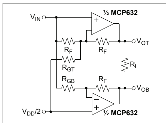
FIGURE 4-12: H-Bridge Driver.
