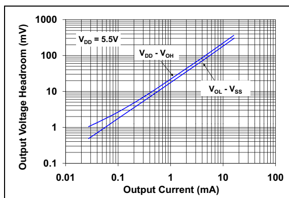
FIGURE 2-24: Output Voltage Headroom vs. Output Current.
