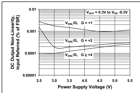
FIGURE 2-8: DC Output Non-Linearity vs. Supply Voltage.
