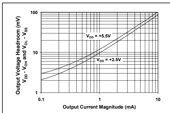
FIGURE 2-21: Output Voltage Headroom vs. Output Current.
