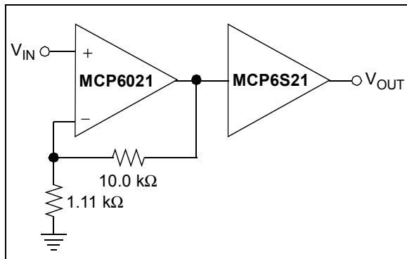
FIGURE 6-4: PGA with Modified Gain Range.
