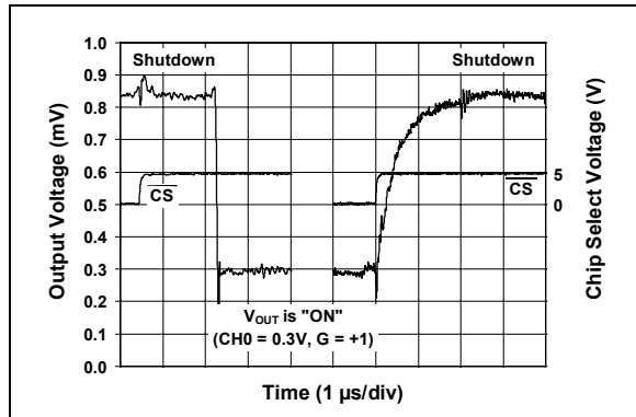
FIGURE 2-31: Output Voltage vs. Shutdown Mode.
