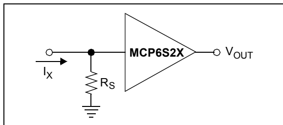
FIGURE 6-3: Wide Dynamic Range Current Measurement Circuit.
