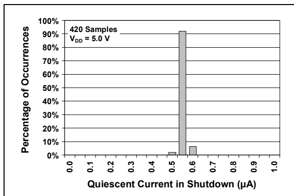
FIGURE 2-20: Histogram of Quiescent Current in Shutdown Mode.
