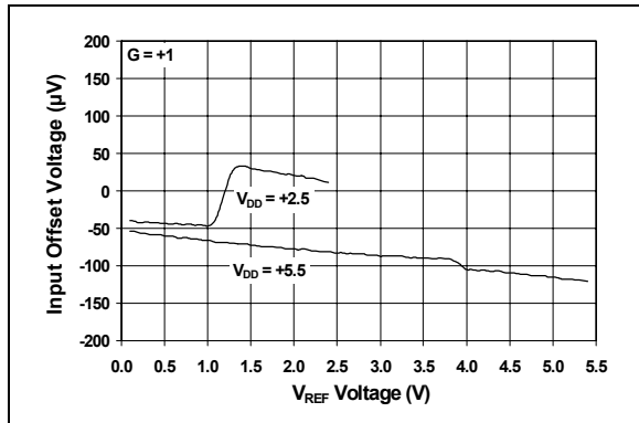
FIGURE 2-7: Input Offset Voltage vs. V_{REF} Voltage.
