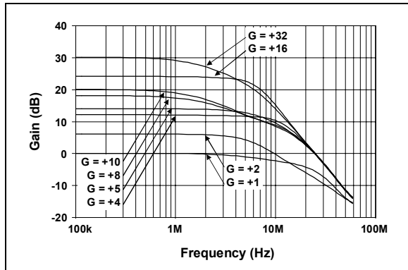
FIGURE 2-19: Gain vs. Frequency.
