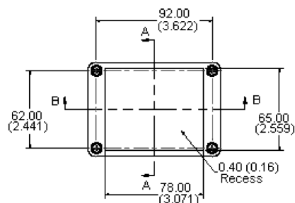
Assembly - Top
