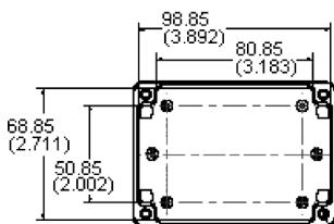
Box - Inside
