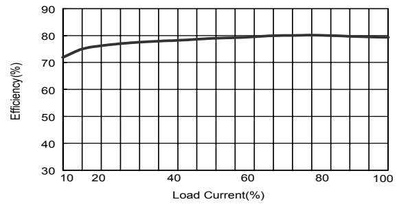
Efficiency vs Output Load
