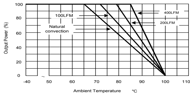
Derating Curve
