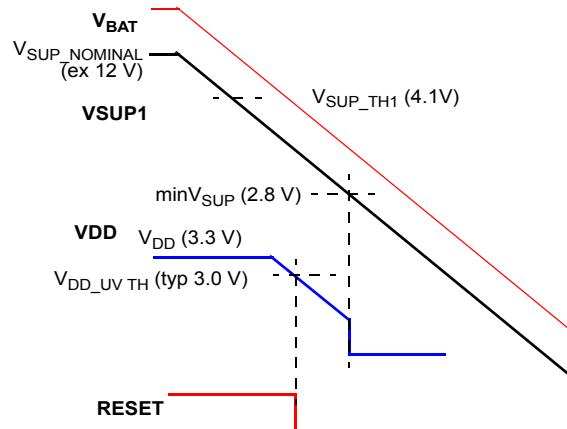
Case 2: V_{DD} 3.3V, " V_{DD} UV TH 3.0 V", with bit Crank = 1
