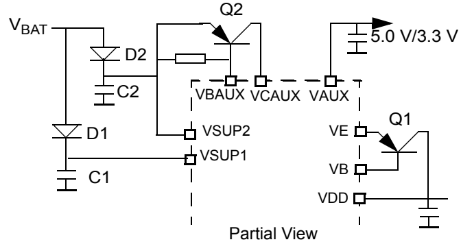
Partial View ex2: Split V_{SUP} Supply
