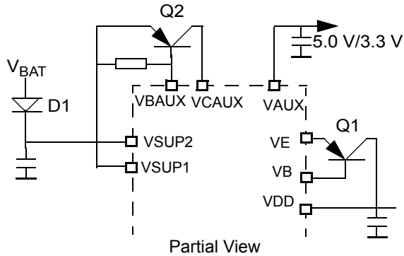
Partial View ex1: Single V_{SUP} Supply
