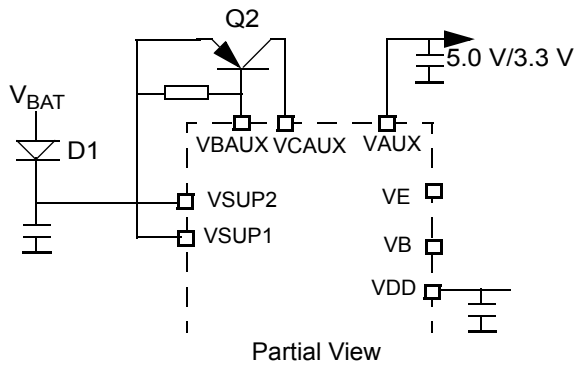
Partial View ex 3: No External Transistor, V_{DD} ~100 mA Capability delivered by internal path transistor.
