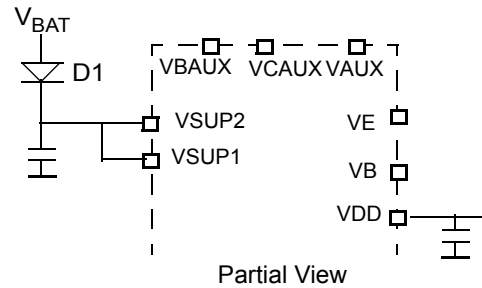
Partial View ex 4: No External Transistor - No VAUX
