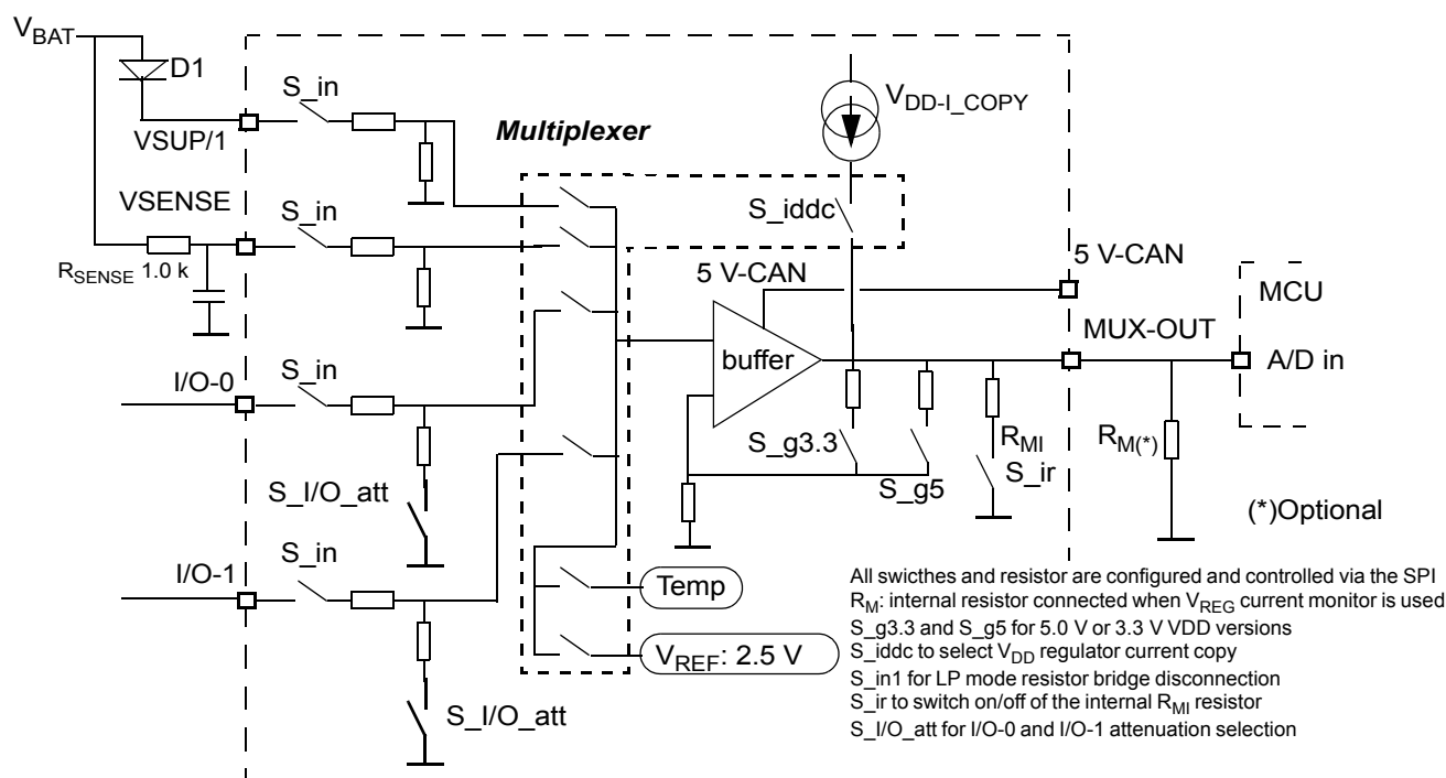
Figure 22. Analog Multiplexer Block Diagram
