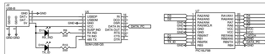
Figure 15: USB Section
