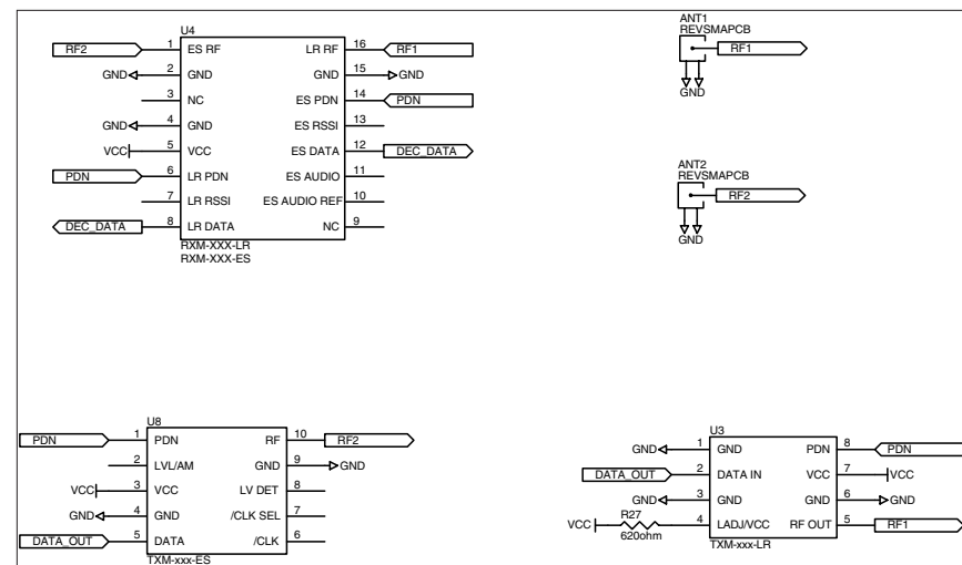
Figure 16: RF Section
