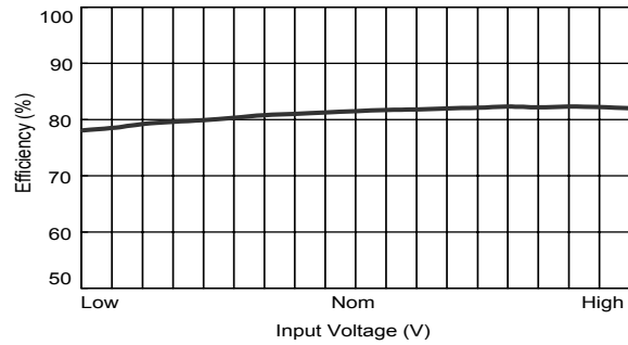
Efficiency vs Input Voltage ( Dual Output )
