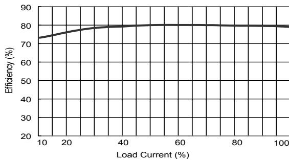
Efficiency vs Output Load ( Single Output )
