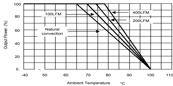
Derating Curve
