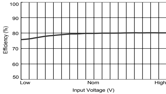
Efficiency vs Input Voltage ( Single Output )
