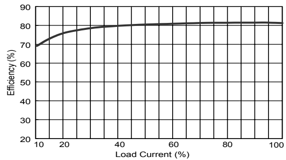
Efficiency vs Output Load ( Dual Output )
