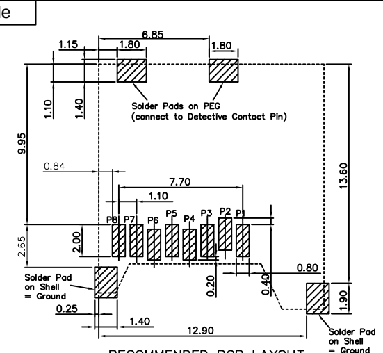
GENERAL TOLERANCE: \pm 0.05
