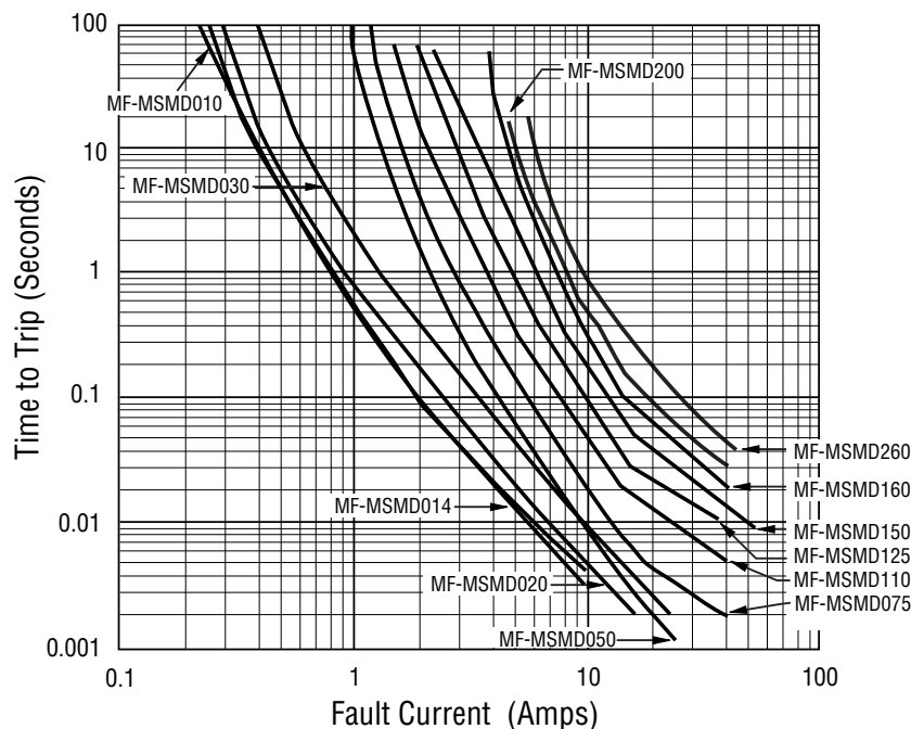
Typical Time to Trip at 23 °C
