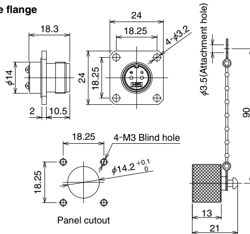
Wide flange
