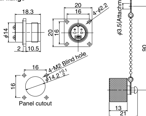
Wide flange
