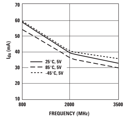
Figure 21. I_{ds} vs. Frequency. ( P_{in} = -10 dBm, V_d = 5 V)
