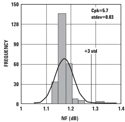
Figure 2. NF @ 2 GHz 3V 40 mA. USL=1.8, Nominal=1.17.
