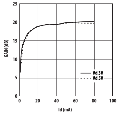
Figure 28. Gain vs. Id (900 MHz).
