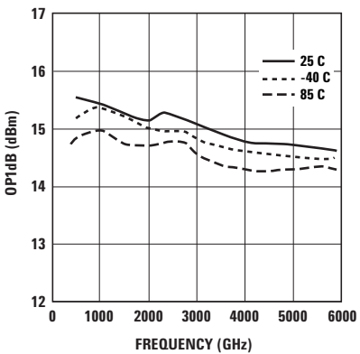
Figure 11. OP1dB vs. Frequency (3V 40 mA).
