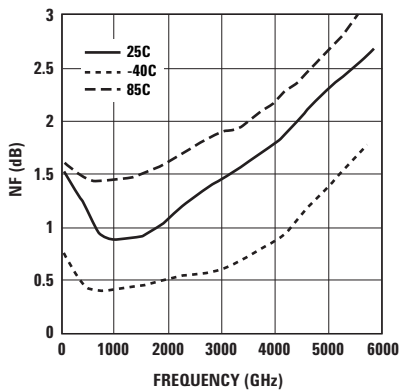
Figure 9. NF vs. Frequency (3V 40 mA).
