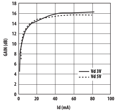
Figure 24. Gain vs. Id (2 GHz).
