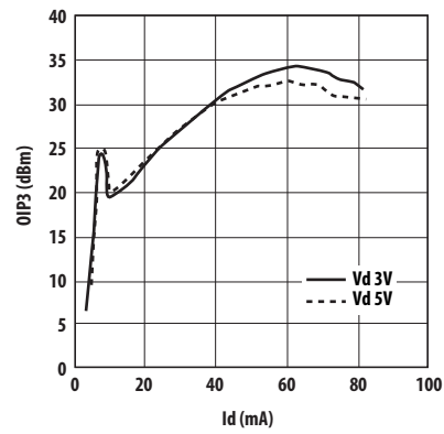
Figure 30. OIP3 vs. Id (900 MHz).
