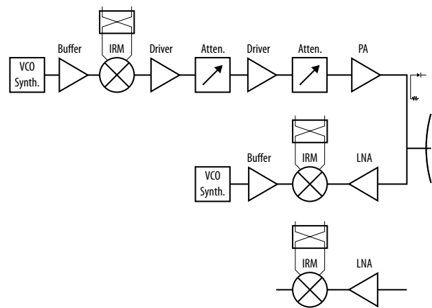
Microwave Link Packaged Suggested Solution 7-8 GHz
