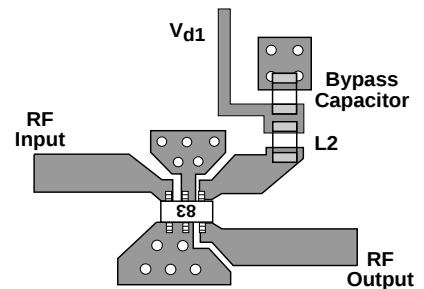
Figure 21. Basic PCB Layout.
