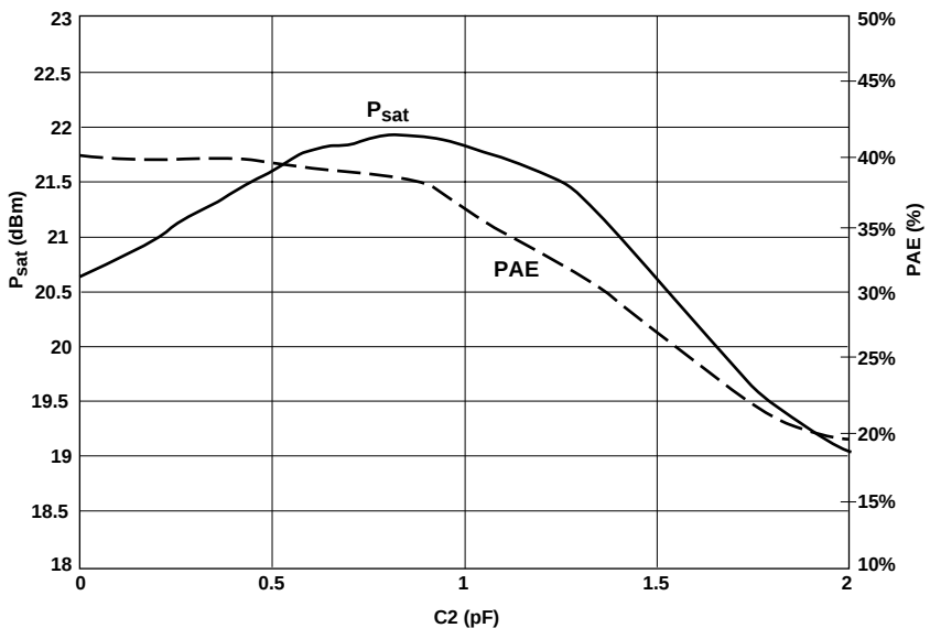
Figure 32. 2.5 GHz P_{sat} and PAE vs. C2.
