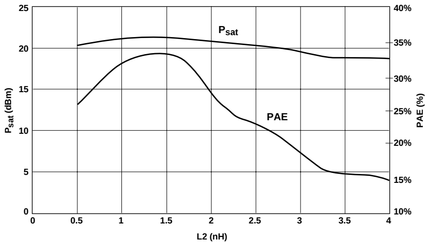
Figure 31. 2.5 GHz P_{sat} and PAE vs. L2.
