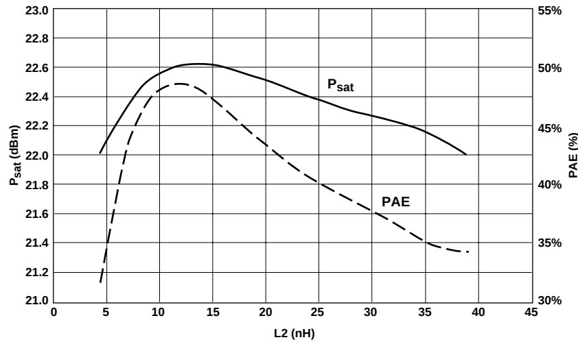
Figure 37. 900 MHz P_{\text{sat}} and PAE vs. L2.
