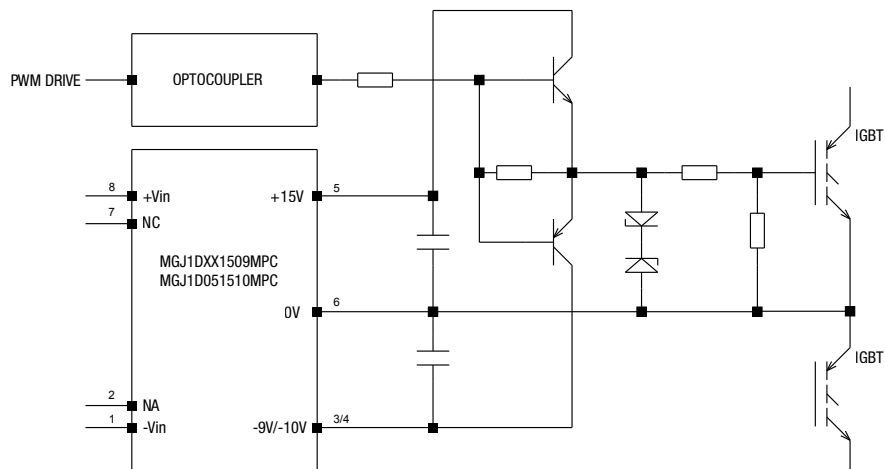
MGJ1 DC-DC CONNECTIONS FOR DRIVING SiC DEVICES
