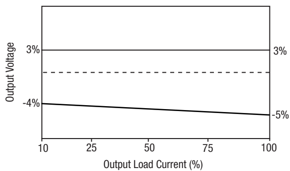
151505, 151509, 151905
