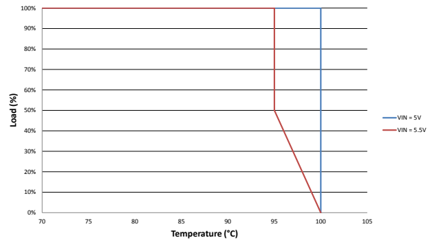
MGJ1D051510MPC
