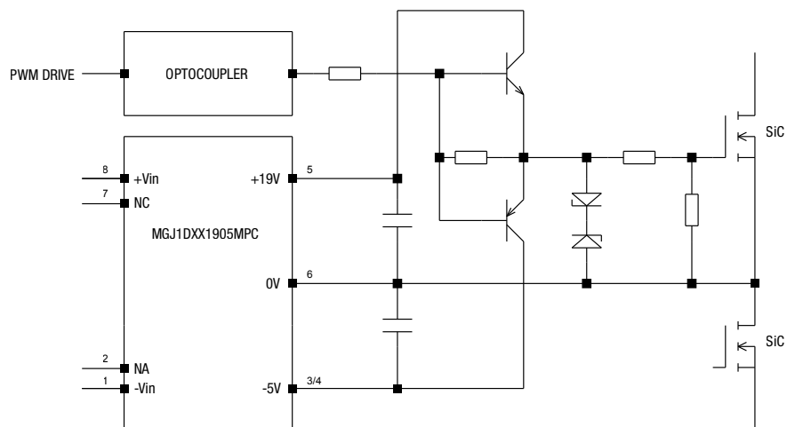
MGJ1 DC-DC CONNECTIONS FOR DRIVING MOSFET DEVICES
