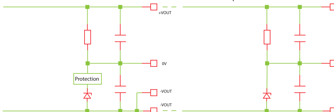
External Zener Diode Network Circuit Option 2
