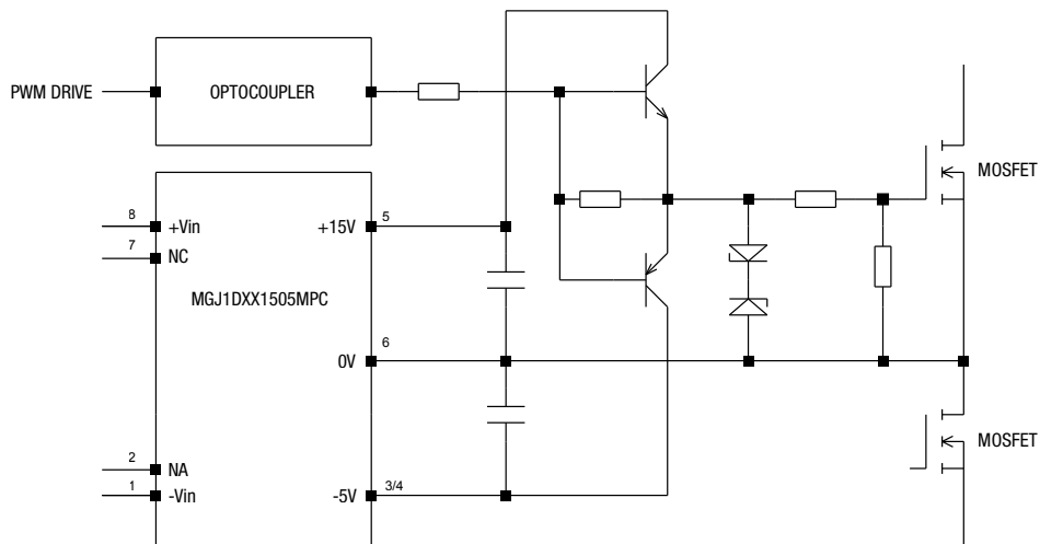
MGJ1 DC-DC CONNECTIONS FOR DRIVING MOSFET DEVICES
