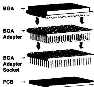
Before Soldering
