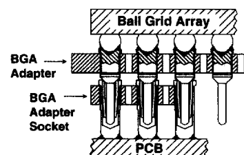
After Soldering
