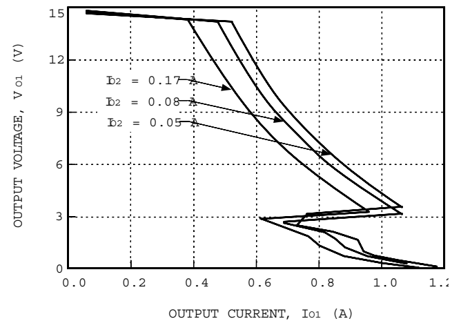
Figure 8. MH005CL Typical Output Characteristics with V_i = 5 V and T_A = 25 °C
