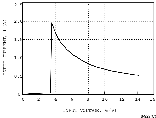
Figure 1. MH005-Series Typical Input Characteristics with I_o = I_{o, \max} and T_A = 25^\circ\text{C}
