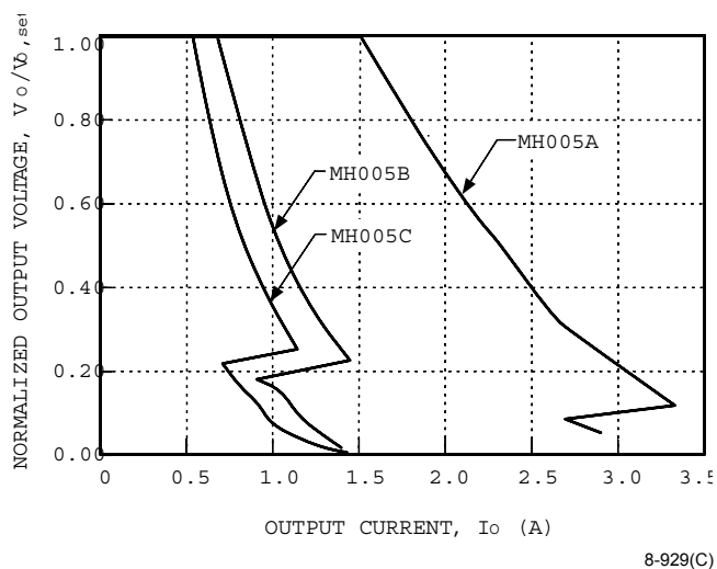
Figure 4. MH005A, B, C Typical Output Characteristics with V_i = 5\text{ V} and T_A = 25^\circ\text{C}
