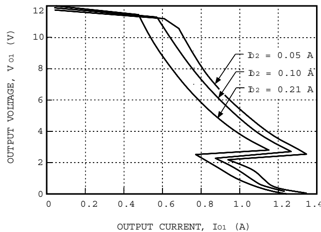
Figure 6. MH005BK Typical Output Characteristics with V_i = 5 V and T_A = 25 °C
