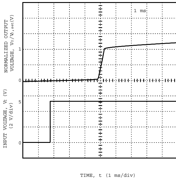
Figure 14. Typical Output Voltage Start-Up when Input Voltage Applied; I_O = 80\% of I_{O, max}
