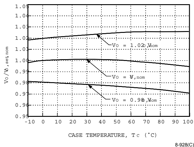
Figure 2. MH005-Series Typical Output Voltage Variation over Operating Case Temperature
