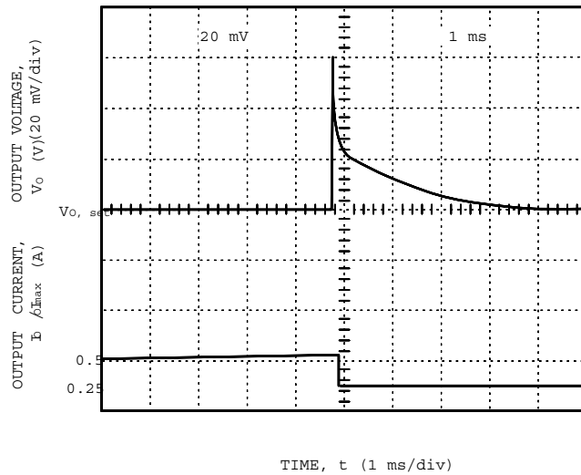
Figure 13. Typical Output Voltage for a Step Load Change from 50% to 25%
