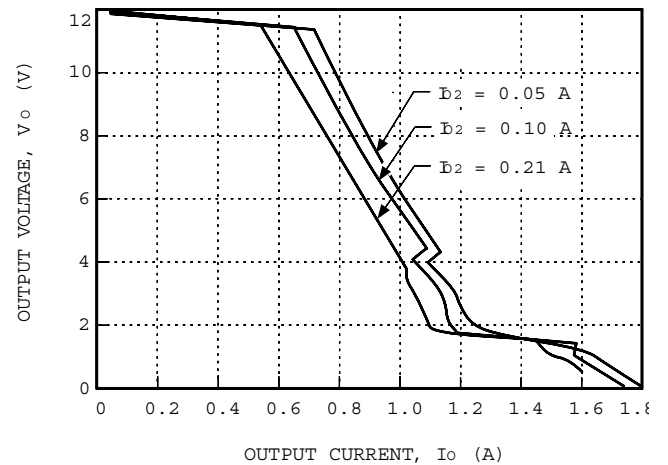
Figure 7. MH005BK Typical Output Characteristics with V_i = 12 V and T_A = 25 °C
