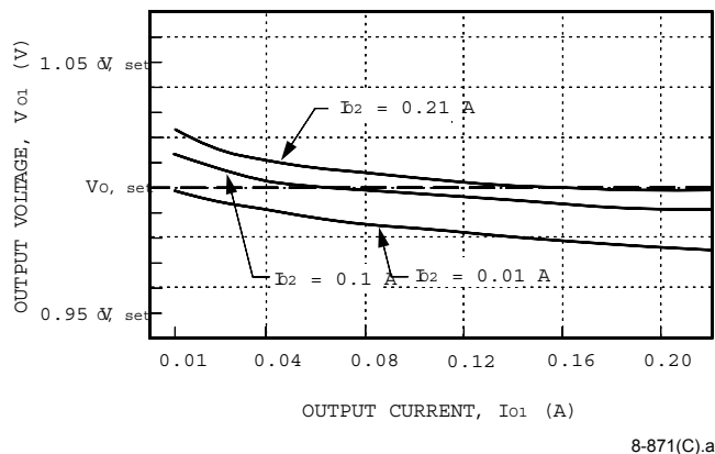
Figure 3. MH005BK, CL Typical V_o vs. I_o Regulation with V_i = 5\text{ V} and T_A = 25^\circ\text{C}
