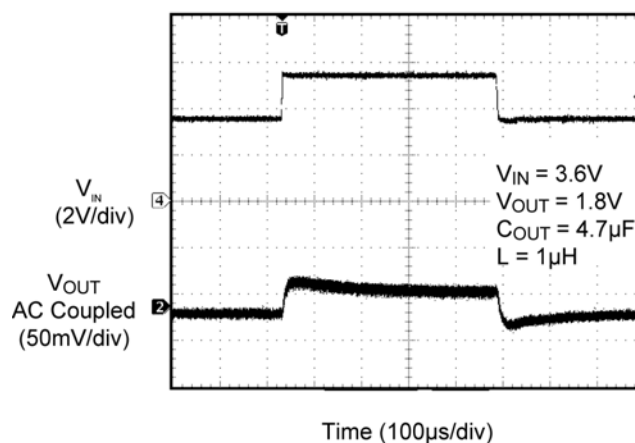
Line Transient (3.6V to 5.5V at 1.5A)
