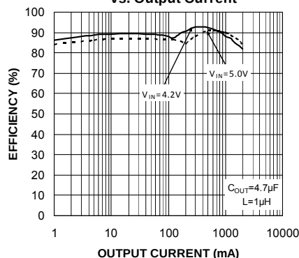
Efficiency ( V_{OUT} = 3.3V ) vs. Output Current
