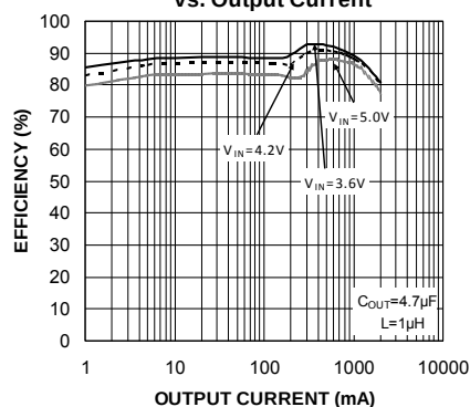
Efficiency ( V_{OUT} = 2.5V ) vs. Output Current
