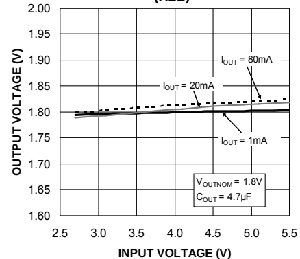
Line Regulation (HLL)
