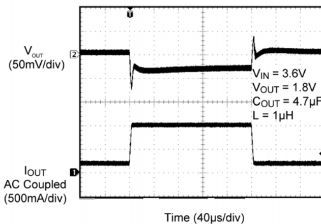
Load Transient (200mA to 1A)
