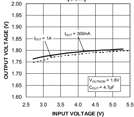
Line Regulation (CCM)
