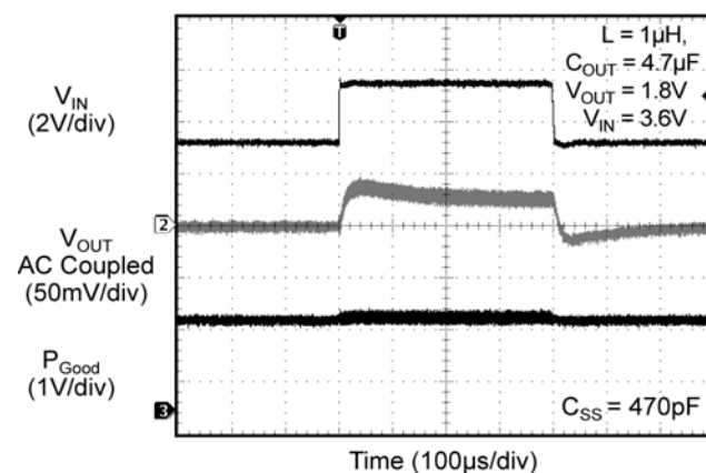
Power Good during Line Transient
