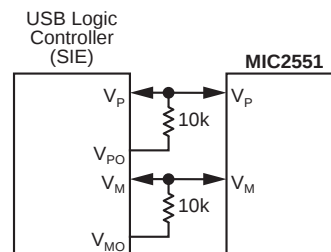
Figure 8. MIC2551 Interface to Non-Multiplexed Data Bus
