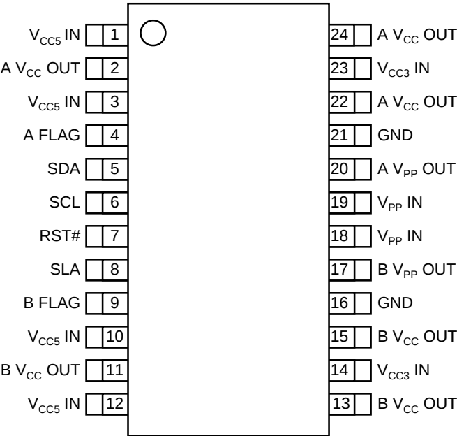
24-lead SSOP (SM)
