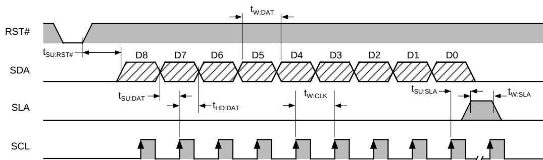
Figure 1. Serial Control Timing Diagram
