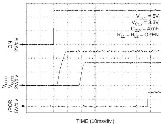
Turn-On, Staggered Mode (MIC2585-1BTS)
