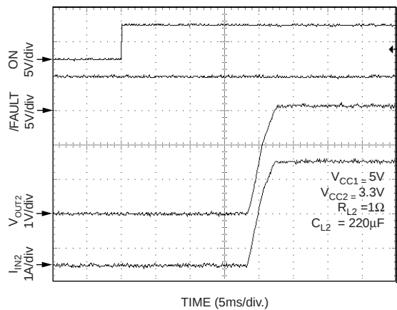
Turn-On (Channel 2)
