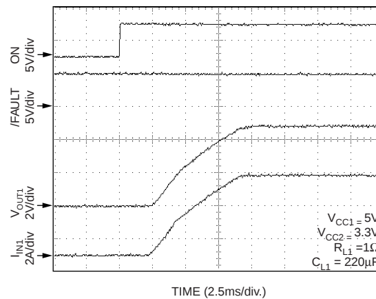
Turn-On (Channel 1)
