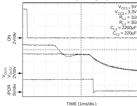
Turn-Off (Tracking On)
