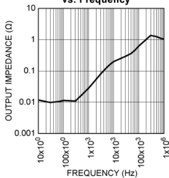
MIC2915x Output Impedance vs. Frequency
