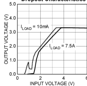
MIC29750-3.3 Dropout Characteristics
