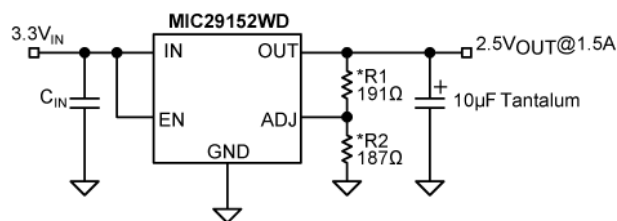
Adjustable Output Voltage
