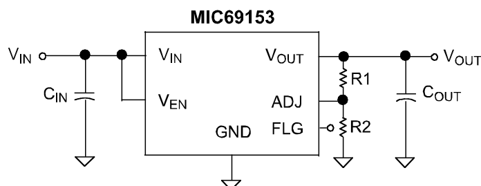
Adjustable Regulator
