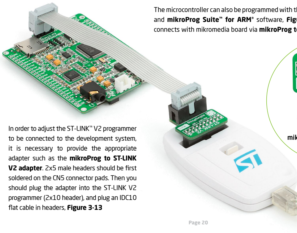
Figure 3-13: Connecting ST-LINK™ V2 programmer
