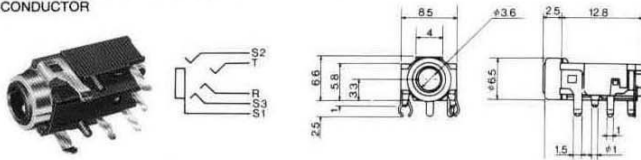
No.M03-428 (φ3.5) 6-CONDUCTOR
