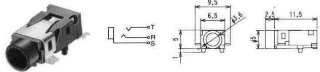
No.M03-292J1 (φ3.5) STEREO
