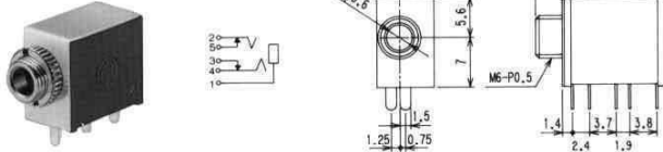
No.MJ-355 (φ3.5) MONO
