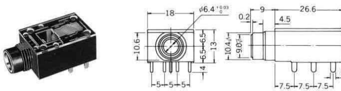
No.MJ-188LP-1~8 PC TYPE 3-CONDUCTOR CIRCUIT 1/4" PHONE JACK Net Weight : 11 gr.
