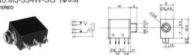
No.MJ-A18 (φ2.5) STEREO
