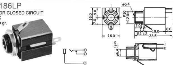
No.MJ-185LP 2-CONDUCTOR OPEN CIRCUIT PHONE JACK Net Weight : 9 gr.
