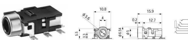
No.MJ-354W-S2 3.5MM STEREO JACK FOR P.C. W/SHIELD HOUSING
