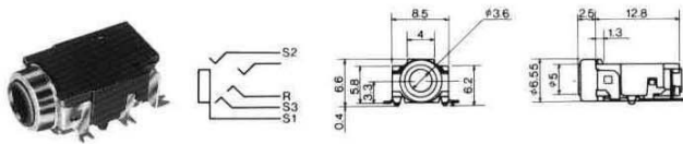
No.MX-385AGM (φ3.5) 5-CONDUCTOR
