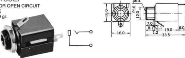
No.MJ-018E 3-CONDUCTOR DOUBLE CLOSED CIRCUIT PHONE JACK Net Weight : 13 gr.
