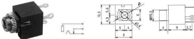
No.MJ-355 (φ3.5) MONO
