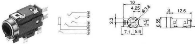
No.M03-721C0 (φ3.5) 6-CONDUCTOR
