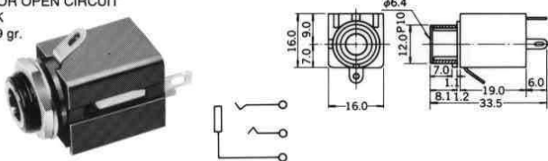
No.MJ-186LP 2-CONDUCTOR CLOSED CIRCUIT PHONE JACK Net Weight : 9 gr.
