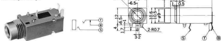
No.MX-617BMB MONO Net Weight : 3.5 gr.
