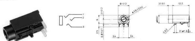
No.M03-681A0 (φ3.5) STEREO
