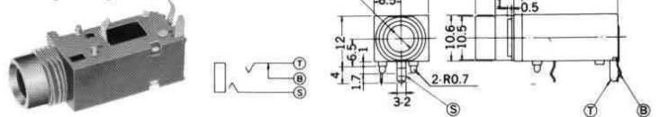
No.MX-616BLB MONO Net Weight : 3.5 gr.
