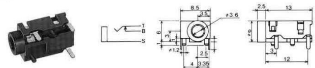
No. MJ-354A0 ( \phi 3.5 )
