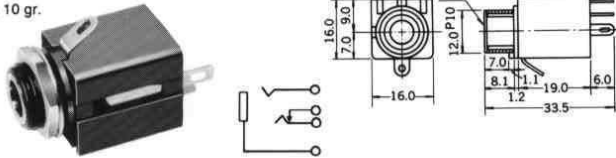
No.MJ-187LP 3-CONDUCTOR OPEN CIRCUIT PHONE JACK Net Weight : 9 gr.
