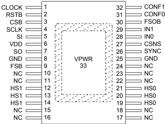
Figure 3. Device Pin Assignments
