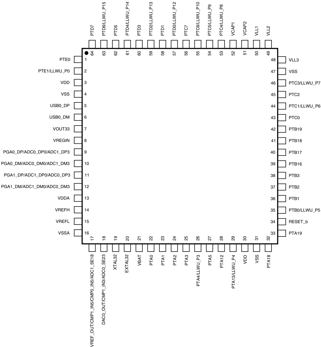
Figure 27. K40 64 LQFP/QFN Pinout Diagram
