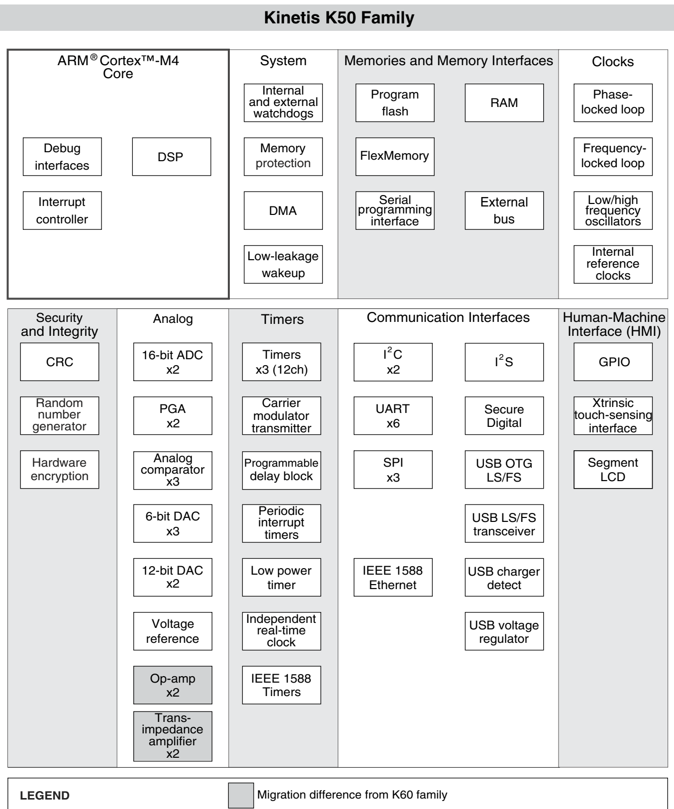
Figure 2. K50 Block Diagram
