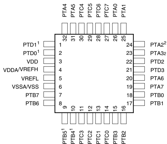
Figure 23. 32-pin LQFP package
