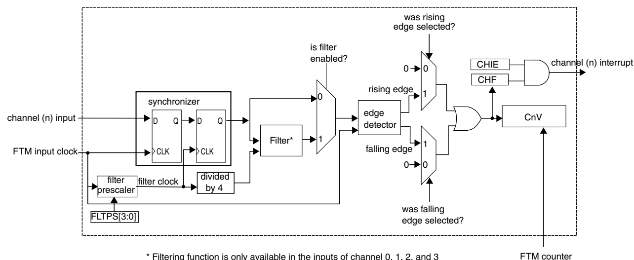
Figure 41-10. Input Capture mode
