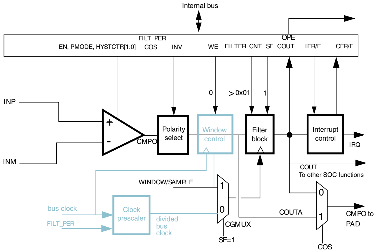
Figure 38-7. Sampled, Filtered (# 4A): sampling point externally driven
