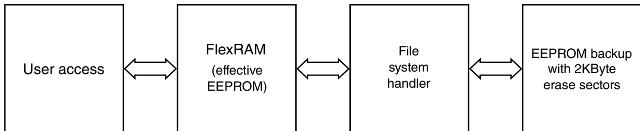
Figure 17-7. Top Level EEPROM Architecture
