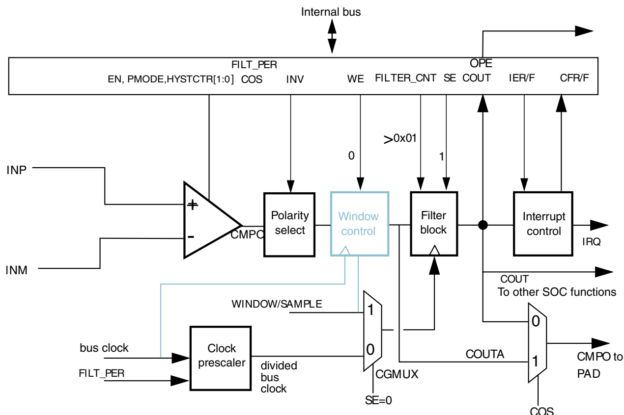
Figure 38-8. Sampled, Filtered (# 4B): sampling point internally derived
