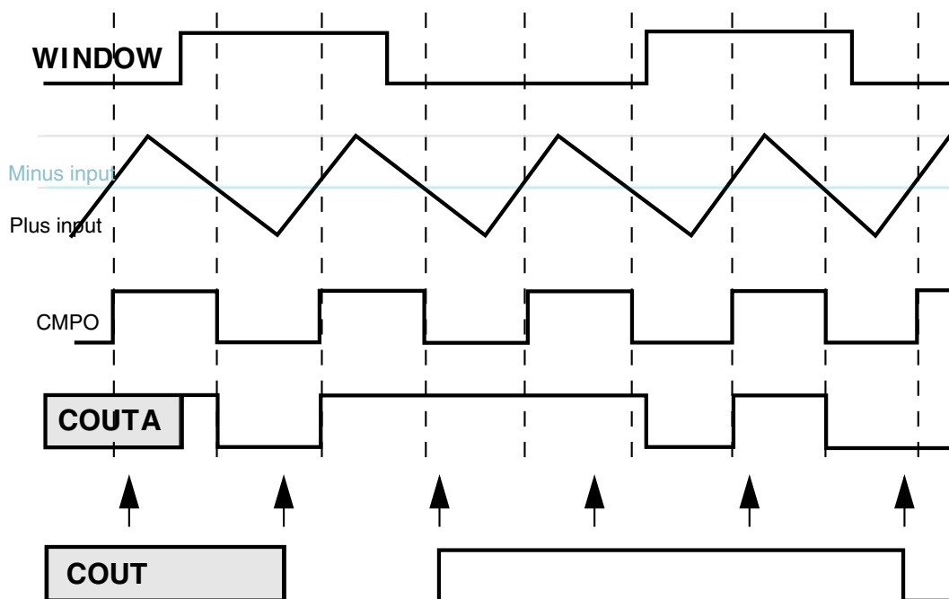
Figure 38-11. Windowed/resampled mode operation
