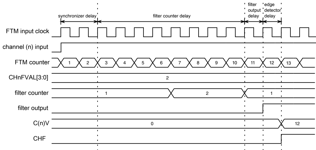
Figure 41-13. Input capture example
