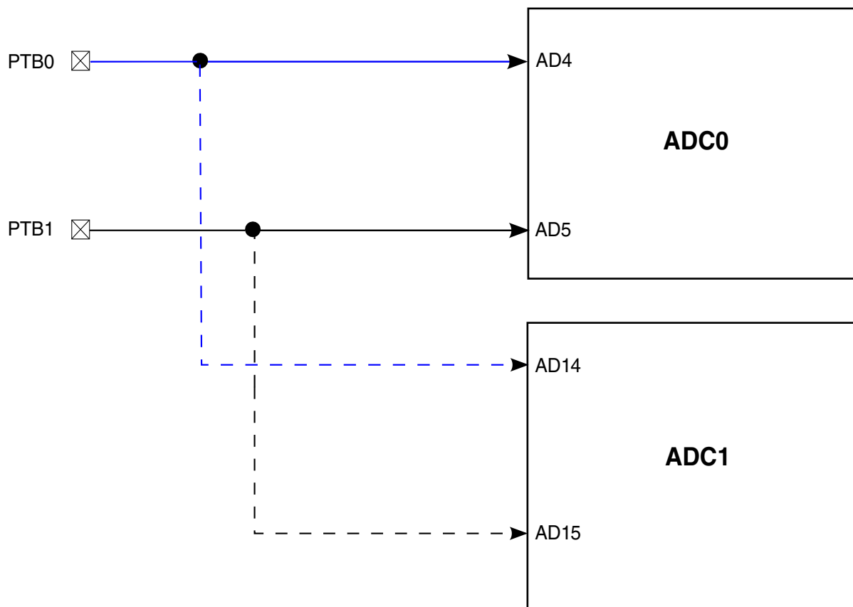
Figure 37-1. ADC0 and ADC1 hardware interleaved channels integration
