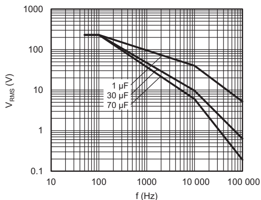
Maximum RMS voltage as function of frequency T_{amb} \leq 85^\circ C ; U_n = 230 V_{AC}
