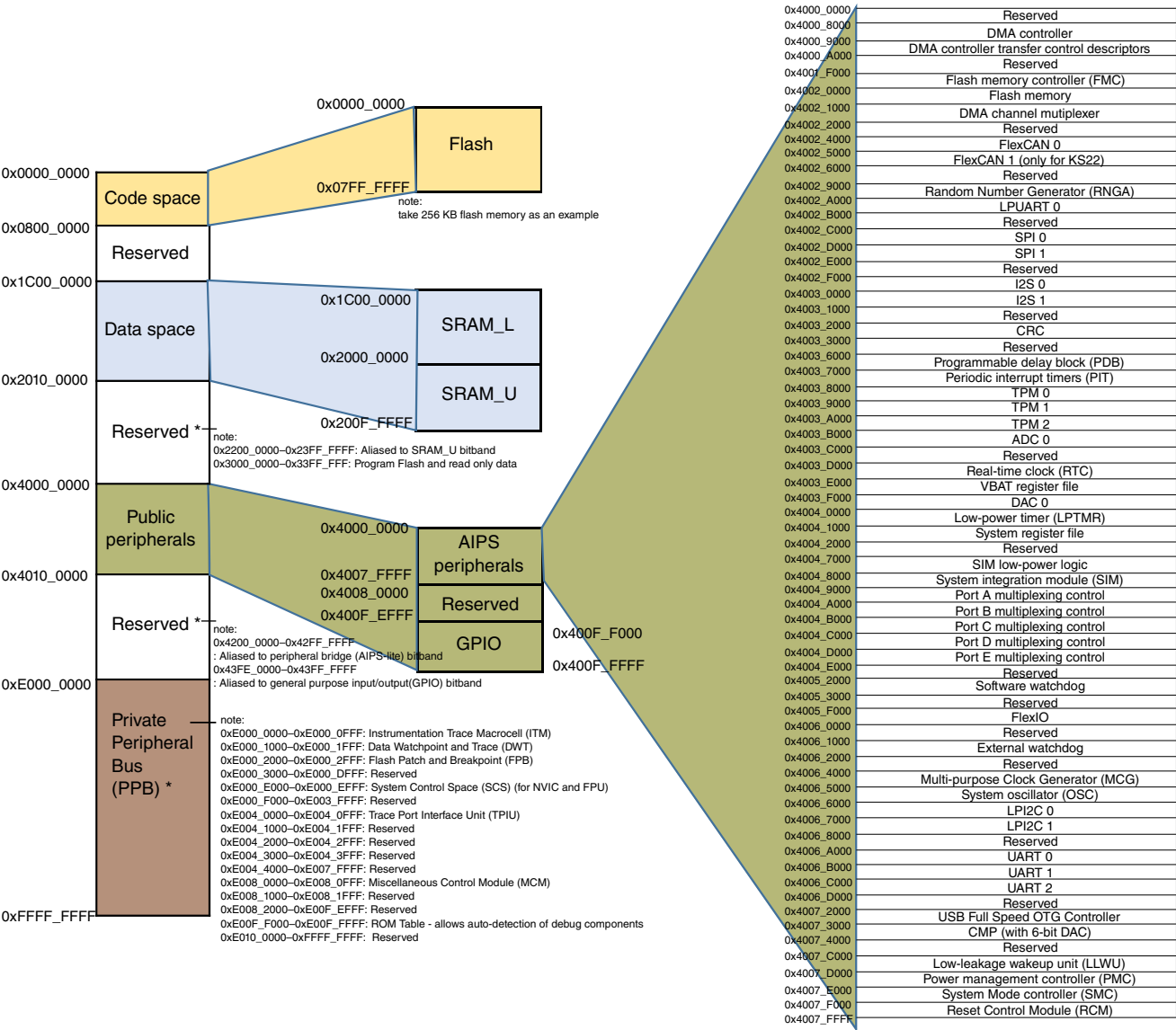
Figure 5. Memory map
