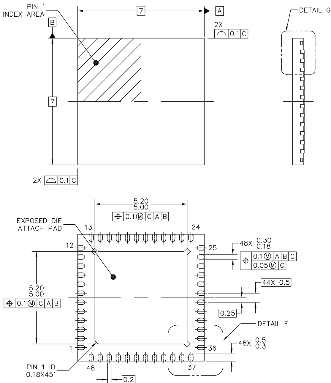
Figure 13. 48-pin QFN package dimension 1
